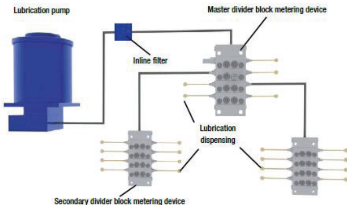
Components of a series progressive automatic lubrication system
