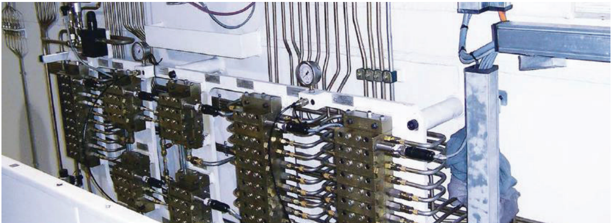
Components of a series progressive automatic lubrication system
